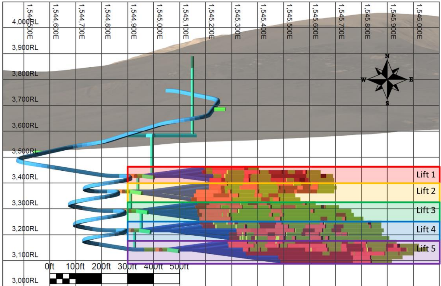
Figure 13-6: Mining Lifts
