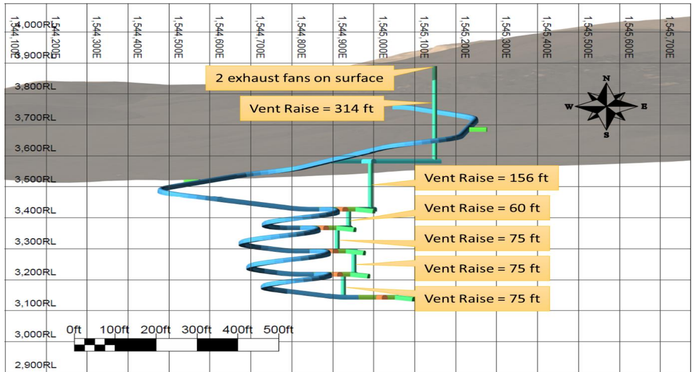
Figure 13-38: Design of Vent Raises
