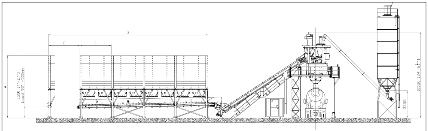
Figure 13-31: Eagle 4000 Backfill Plant
