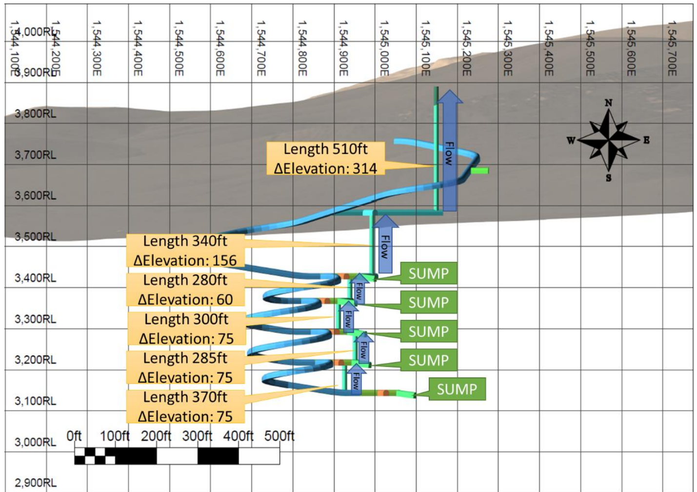
Figure 13-39: Sump Design and Layout
