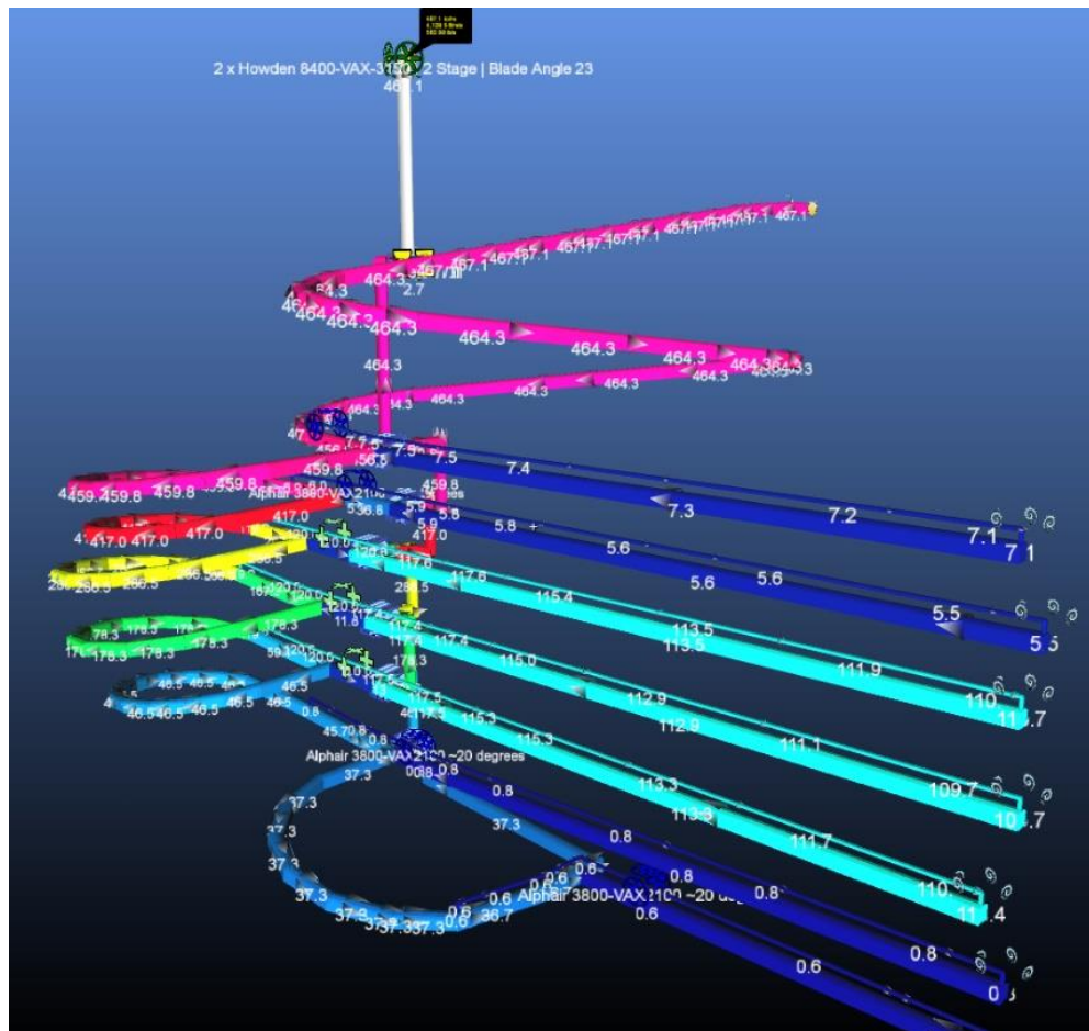
Figure 13-36: Ventilation Network (isometric view looking west)
