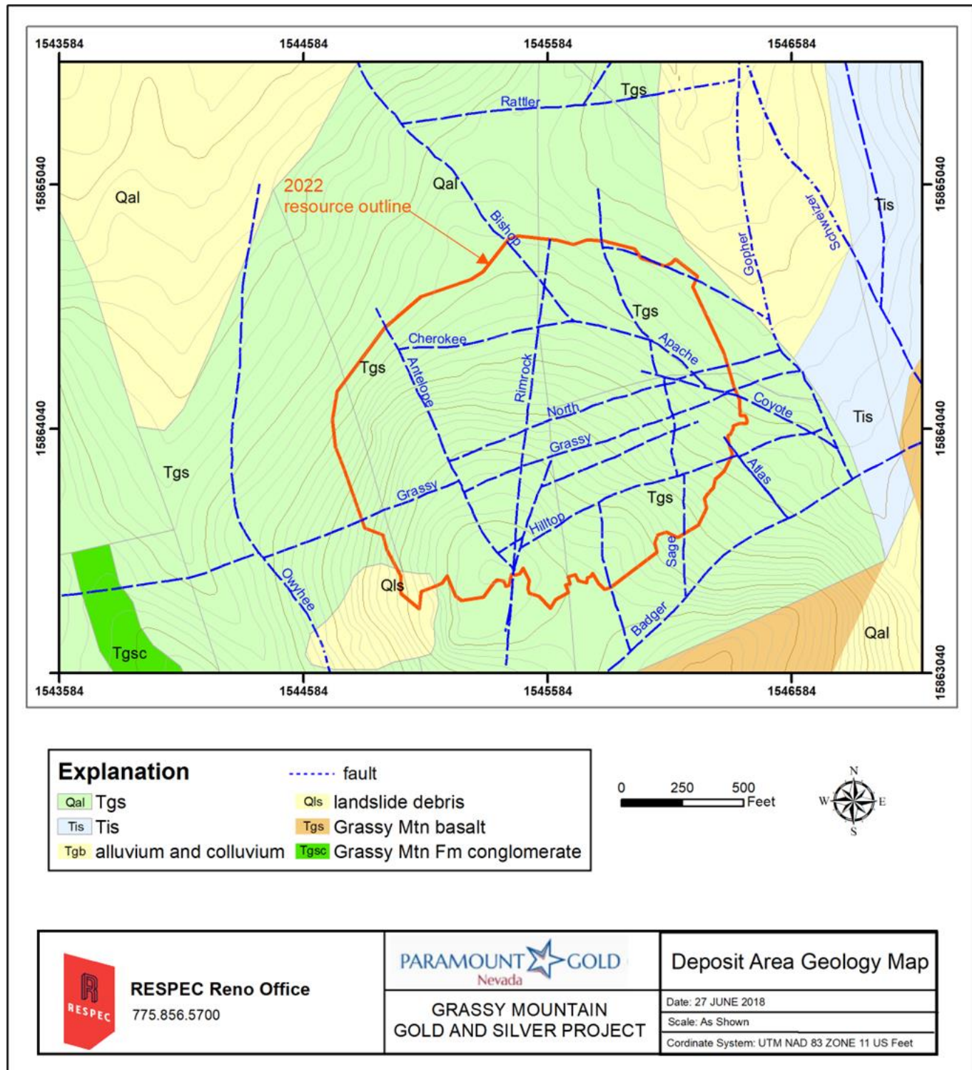
Figure 6-3: Grassy Mountain Deposit Area Geologic Map
