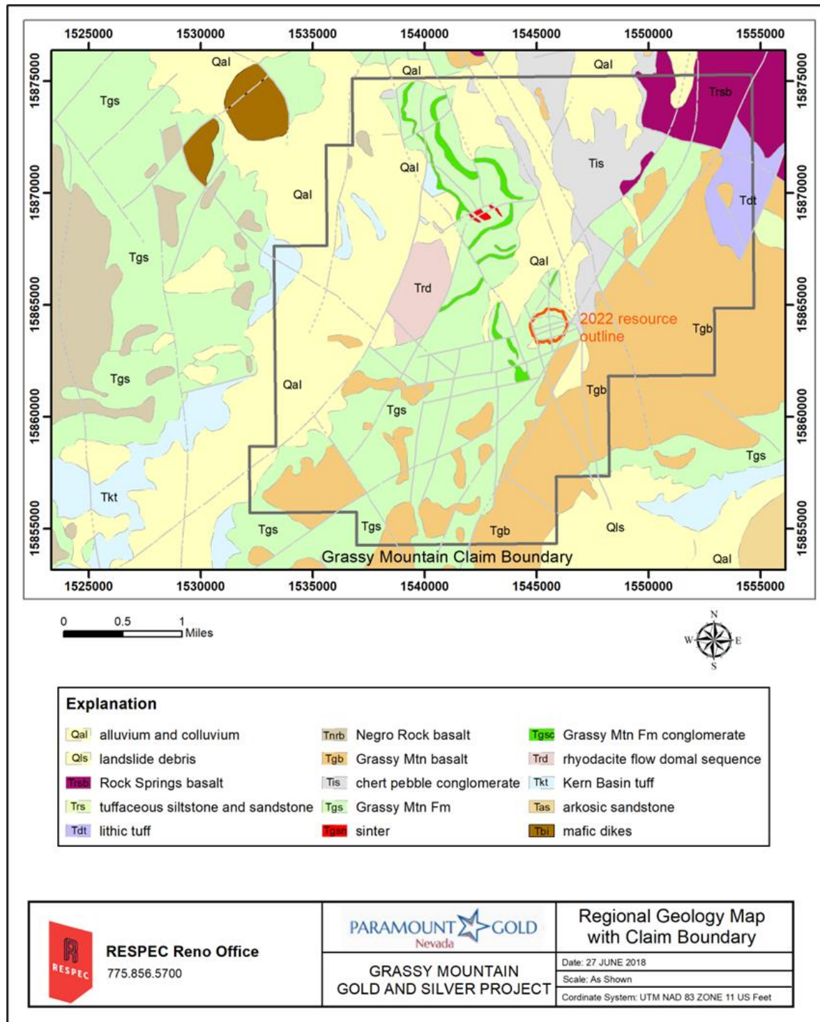
Figure 6-1: Grassy Mountain Regional Geology
