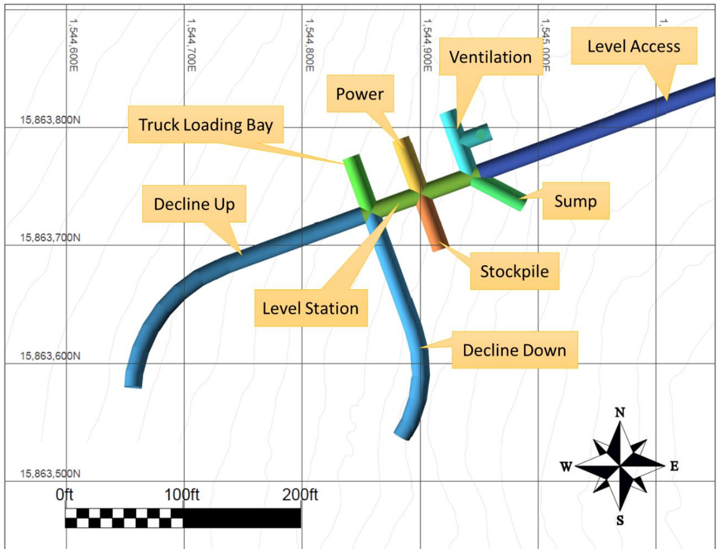
Figure 13-19: Station Design
