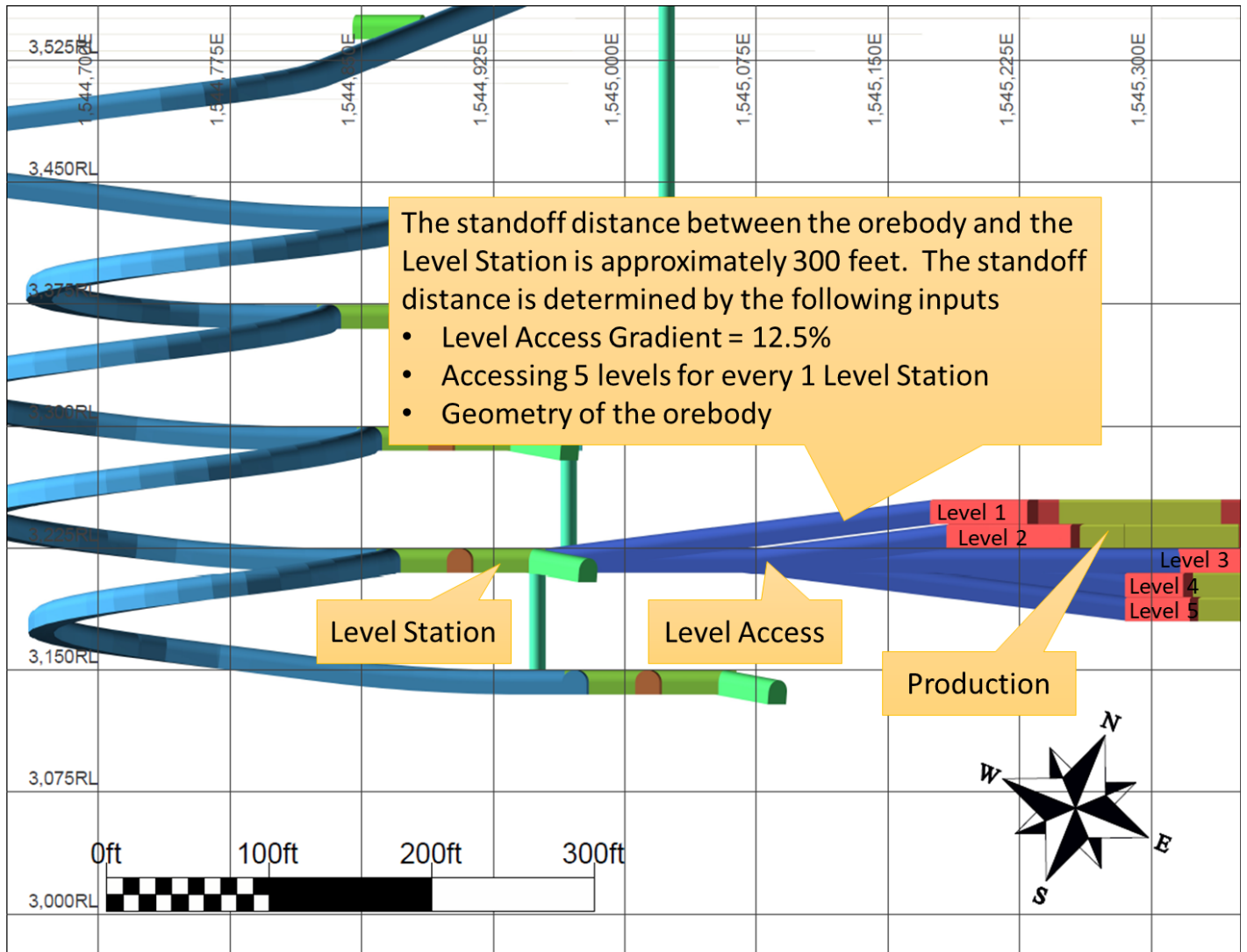
Figure 13-18: Level Access Layout (Looking North)
