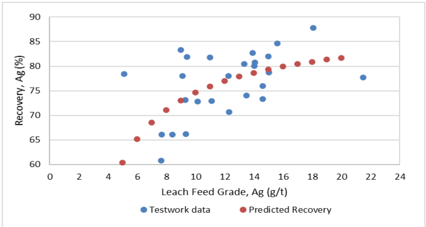
Figure 10-7: Predicted versus Measured Recovery for Silver
