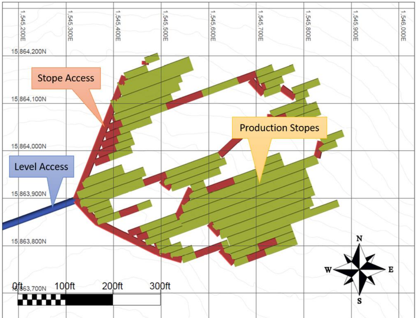
Figure 12-3: Mine Production Design of Level 3210, Plan View
