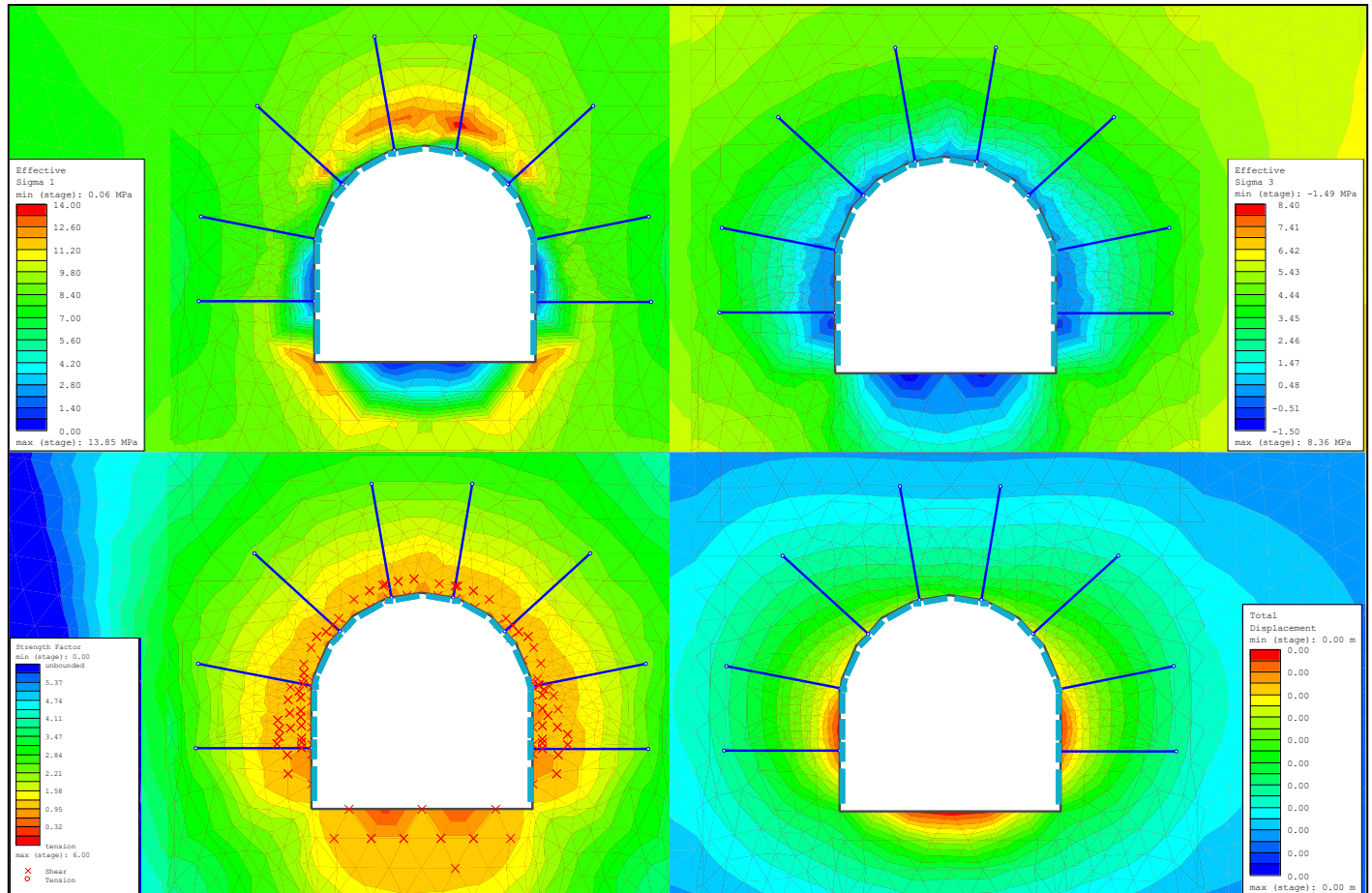
Figure 13-13: Modeling Results for Decline Ramp; a) Major Principal Stress, S1; b) Minor Principal Stress, S3; c) Strength Factor, SF; d) Displacements
