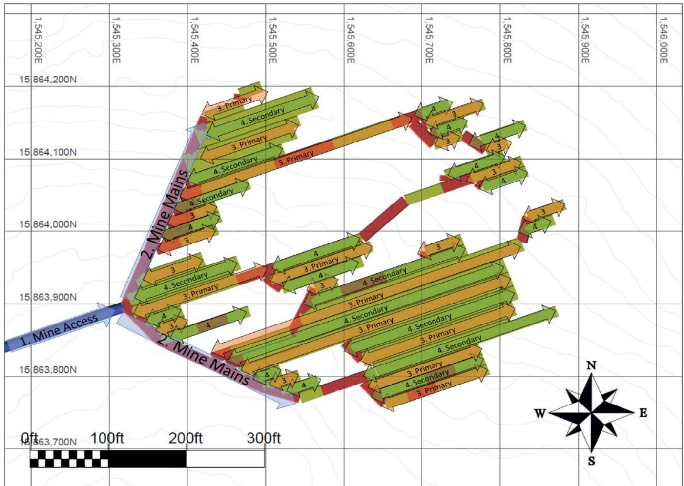
Figure 13-5: Detailed level Sequence for a Typical Level
