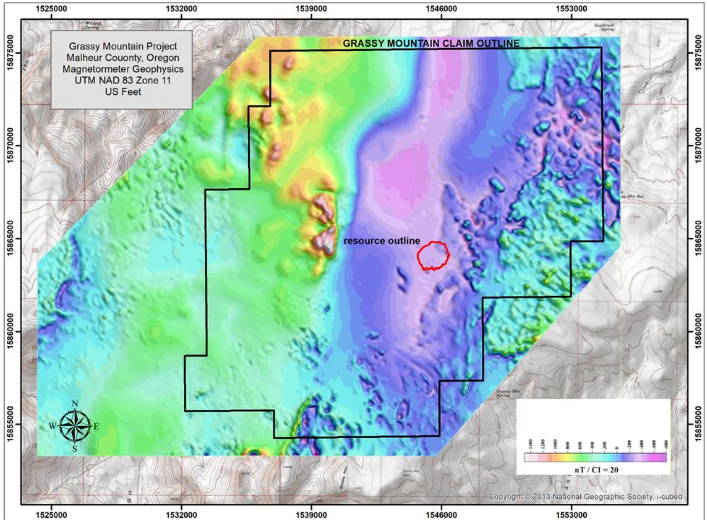
Figure 7-1: 2018 Aerial Magnetic Survey of Grassy Mountain Area
