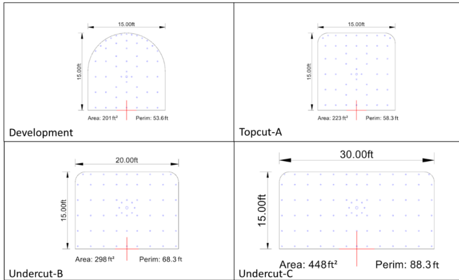
Figure 13-3: Drift Profiles
