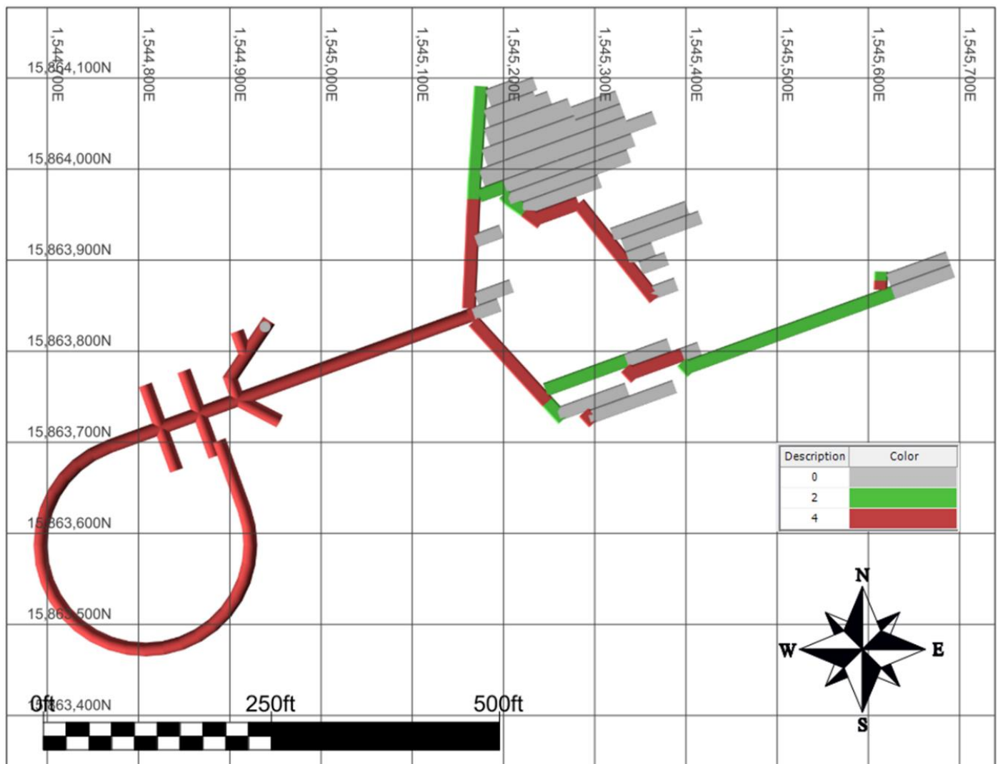
Figure 13-23: 3360 Shotcrete Thickness (units in inches)
