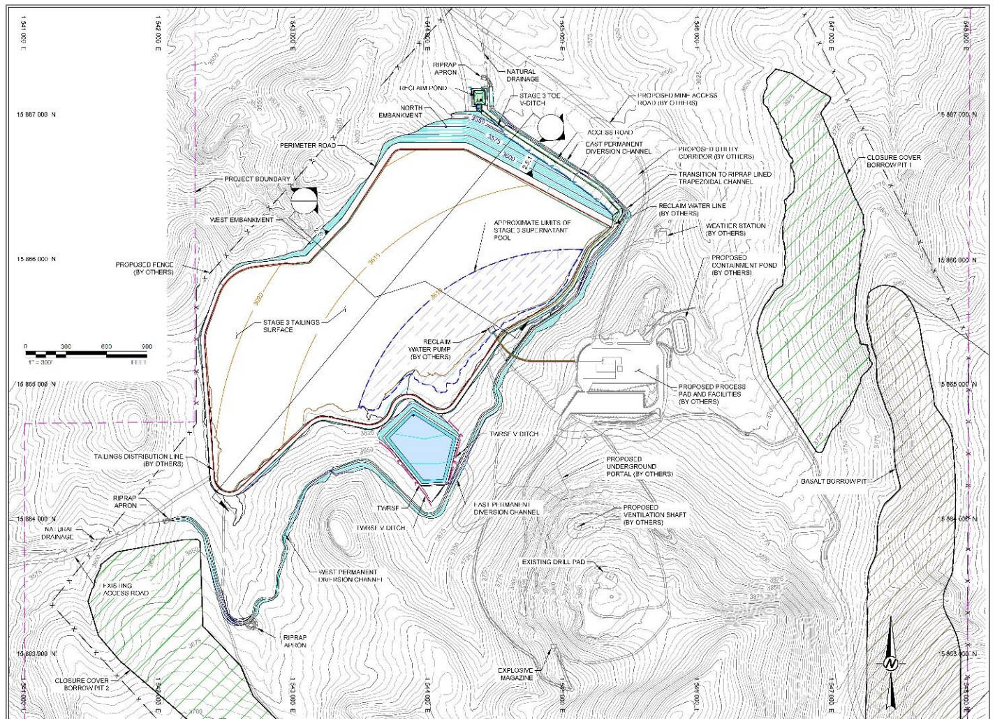
Figure 15-2: Overall TSF Layout
